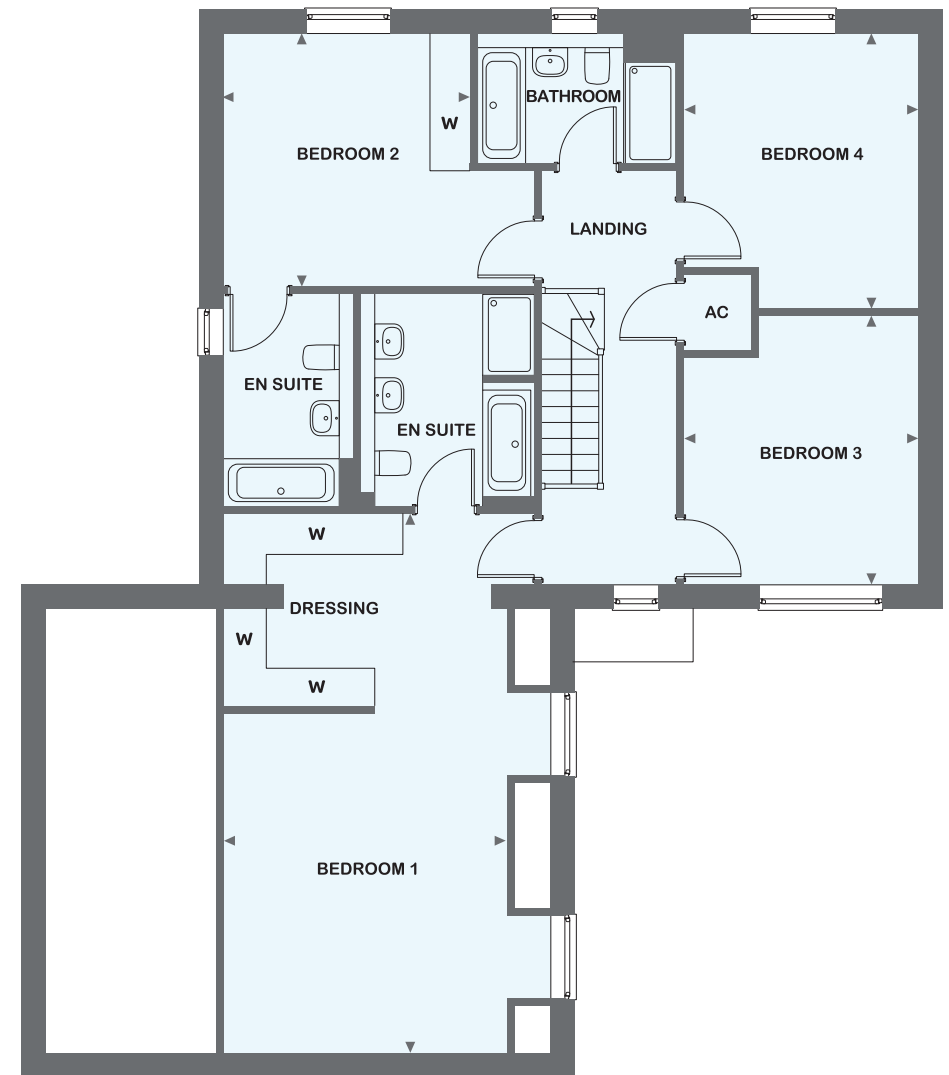
FIRST FLOOR
